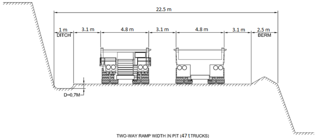
Figure 16-2: Typical In-Pit Dual-Lane Ramp on Rock
