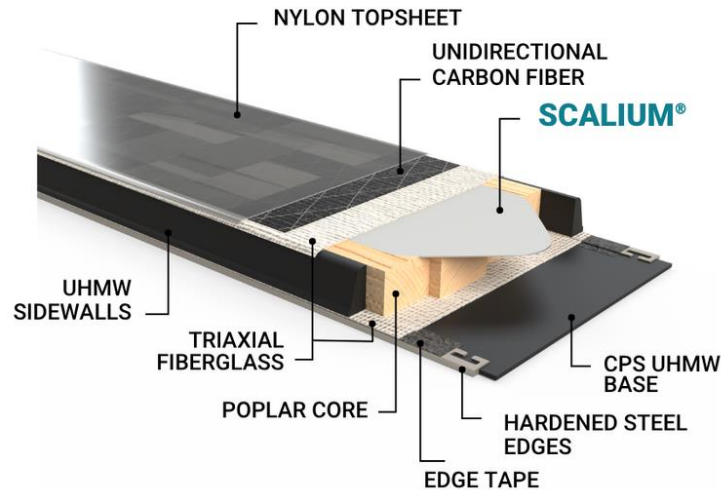
Figure 1: Internal construction of the Ferreol Pionnier 104 2.0 model, featuring a sheet of Scaliu®.
